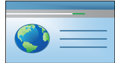
Admin Interface
